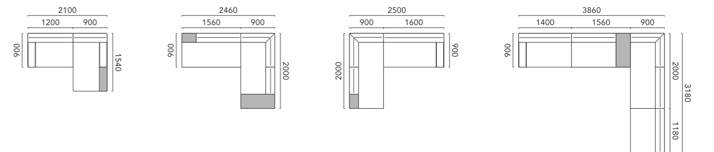
LAYOUT PATTERN
